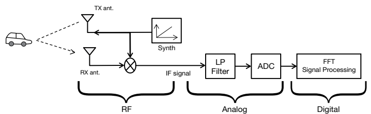
Figure 14. RF, analog and digital components of an FMCW sensor.
