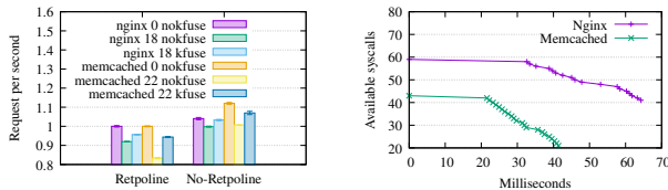
(a) Throughput of NGINX and Memcached with 18 and 22 seccomp filters by incremental tightening. The results are normalized to the baseline, 0 seccomp filters and rtpoline enabled. (b) The number of allowed system calls for NGINX and Memcached over time as incremental tightening blocks system calls during execution.
